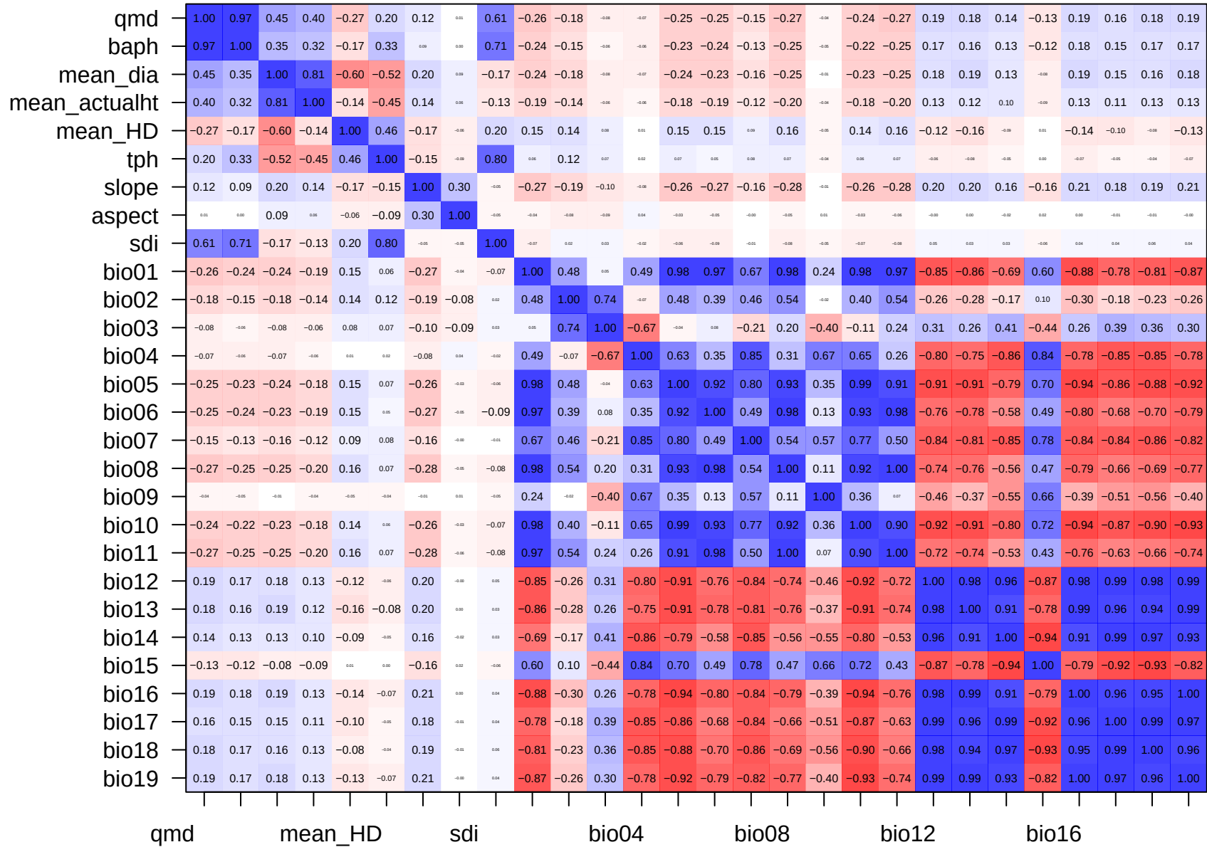
Correlation plot from data
